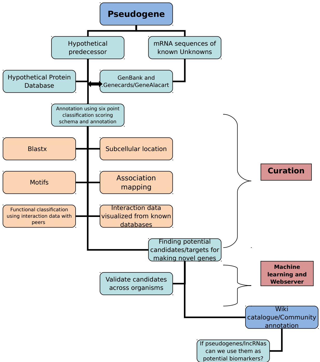
Figure 1: Approaches in developing a webserver of pseudogene prediction. If any candidate genes do exist as pseudogenes, we will make novel proteins (PR Shidhi et al. 2014) which in turn may be used as potential biomarkers.
